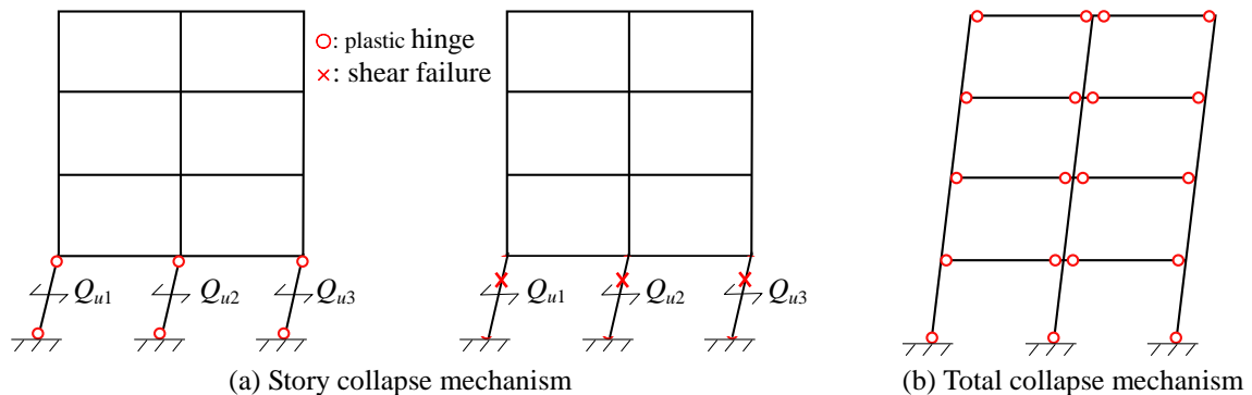
Figure 4. typical collapse mechanism of frame structures
