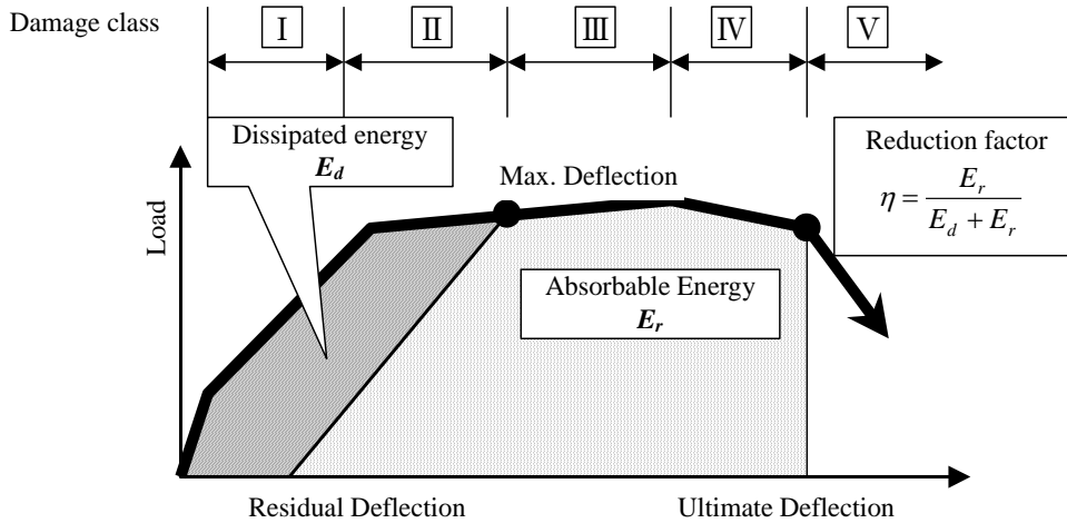
Figure 3. Seismic capacity reduction factor \eta (JBDPA 2001a)
