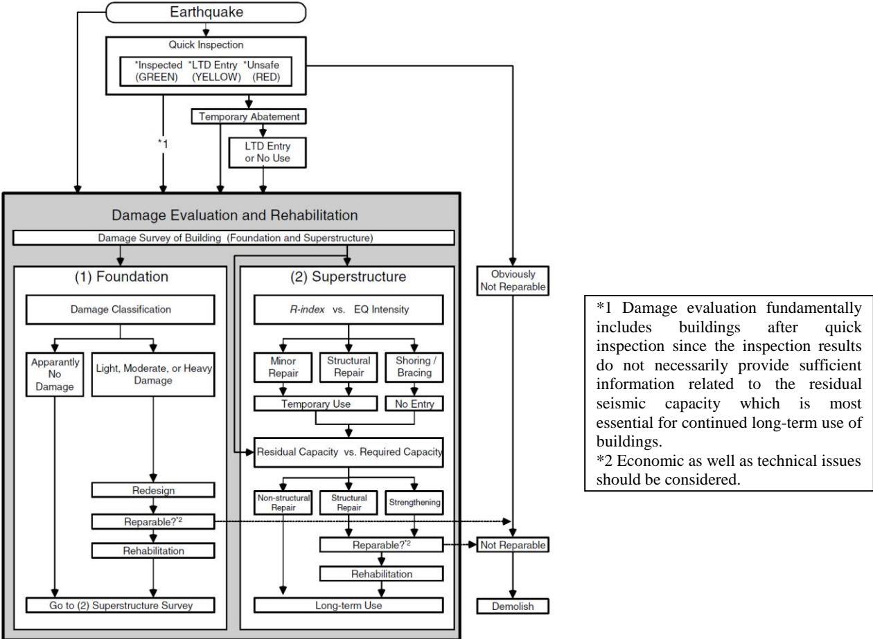
Figure 1. General Flow of Damage Evaluation and Rehabilitation in the Guideline (Nakano et al. 2004)
