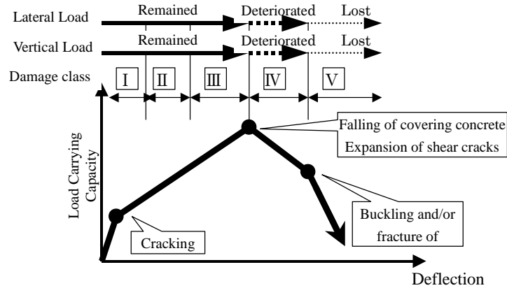
(b) Brittle member
