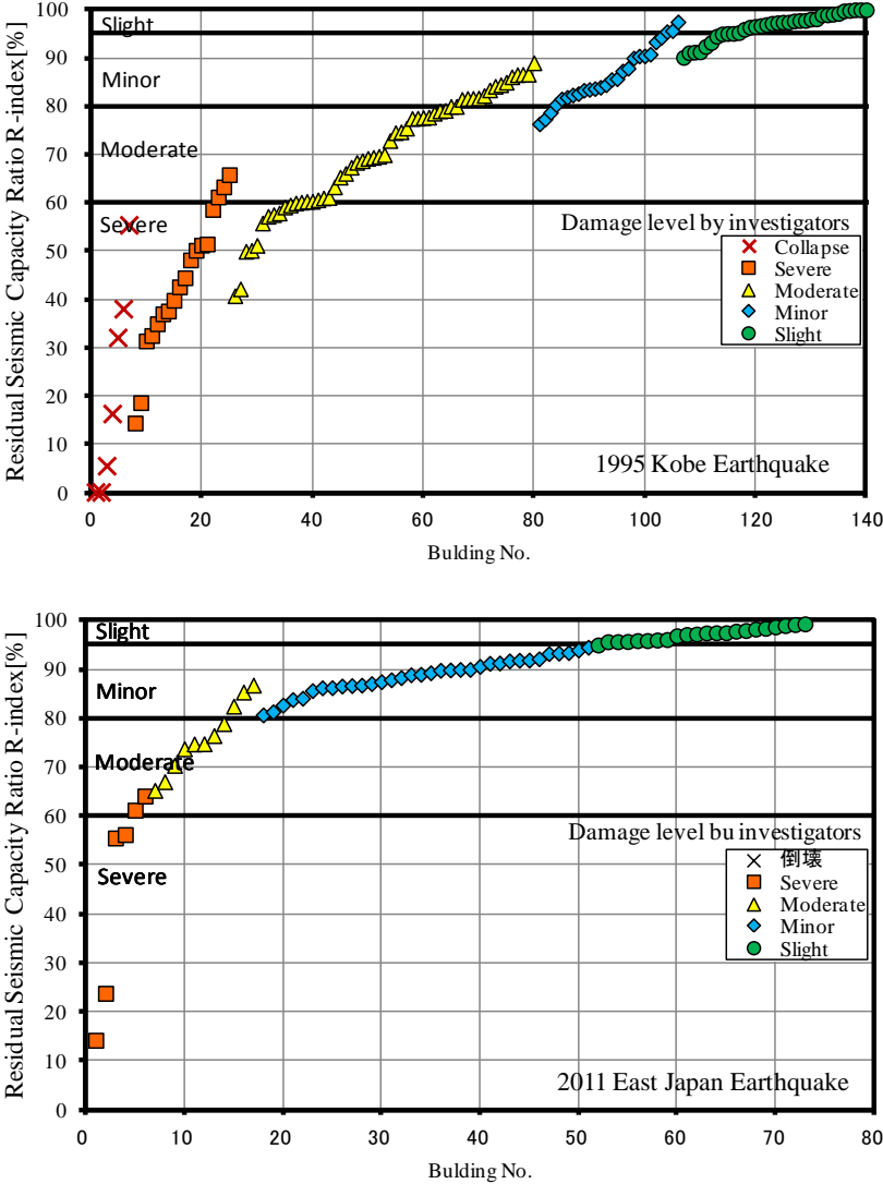
Figure 4 Residual seismic capacity index R and observed damage levels due to Kobe Earthquake.
