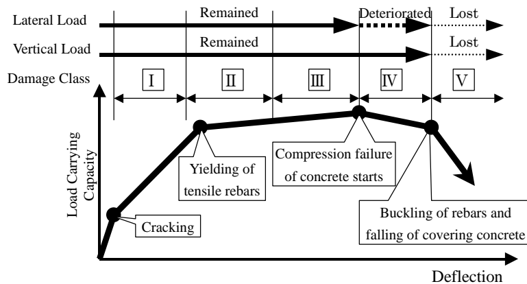
(a) Ductile member
