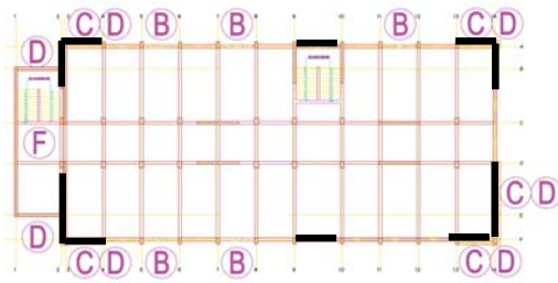
Figure 4. Example of retrofit with new concrete walls
