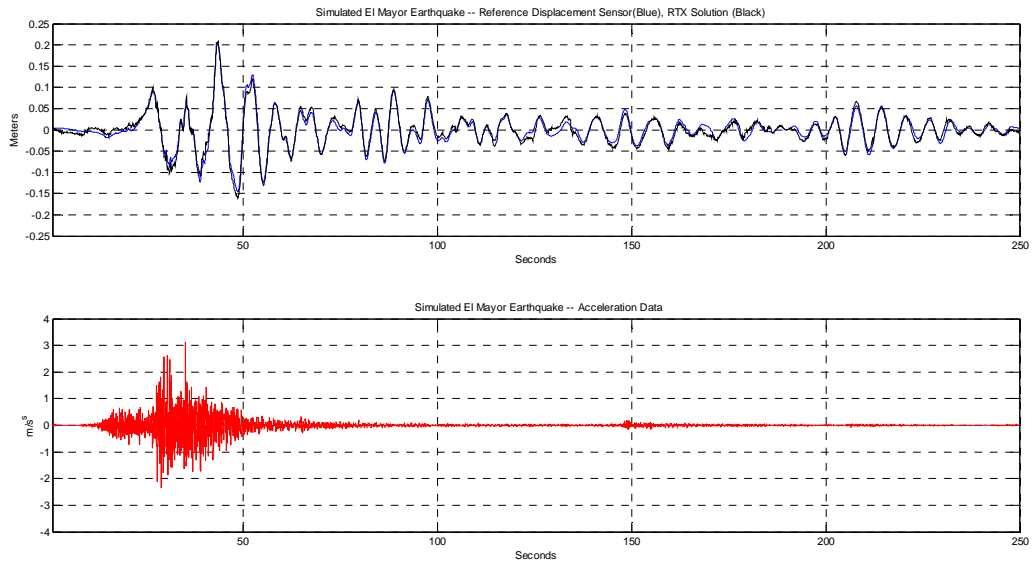
Figure 1: Time series of the reference displacement (blue) and GNSS/RTX (black), and acceleration (red); Sierra El Mayor (Mexico) simulated earthquake.
